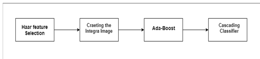
Figure 7-Flow of viola-jones algorithm [12].
