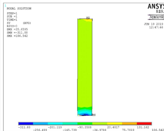
Y Component Solution
