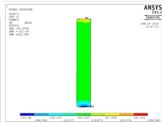
X Component Solution
