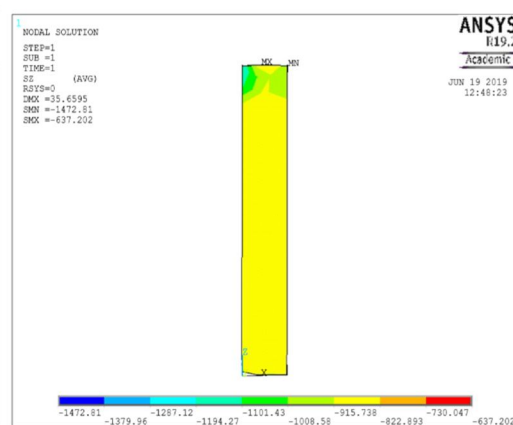
Z Component Solution
