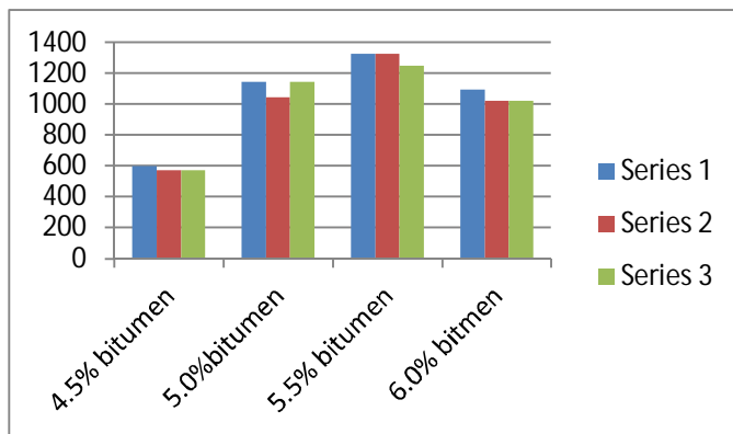
Figure1. Stability values for different mix proportions of bitumen (for OBC)
