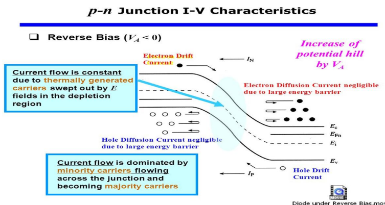
Fig.6.1 Current flow in p-n junction
