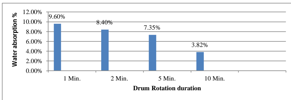
Figure 1 - Water absorption % after abrasion of RA
