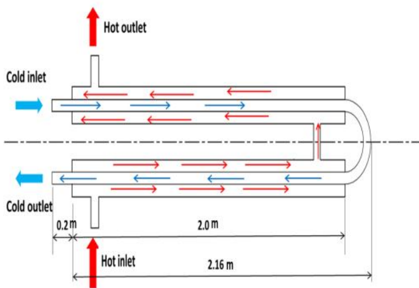
Fig.3: Flow diagram of double pipe heat exchanger
