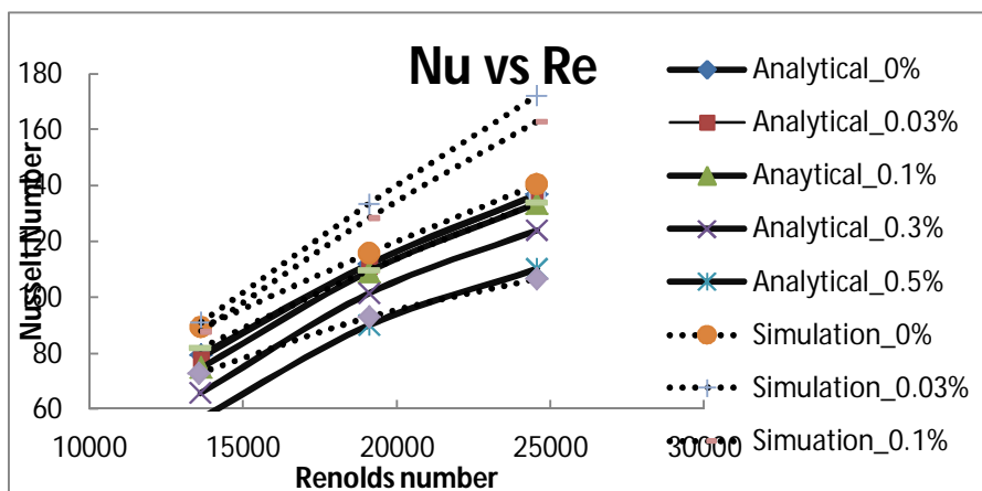
Fig 4: Effect of friction factor on Reynolds number.
