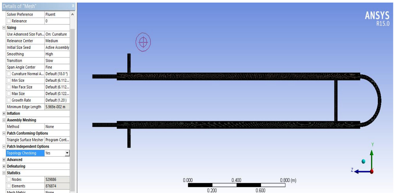
Fig. 1. Meshing of 2 pass double pipe heat exchanger in ANSYS Workbench
