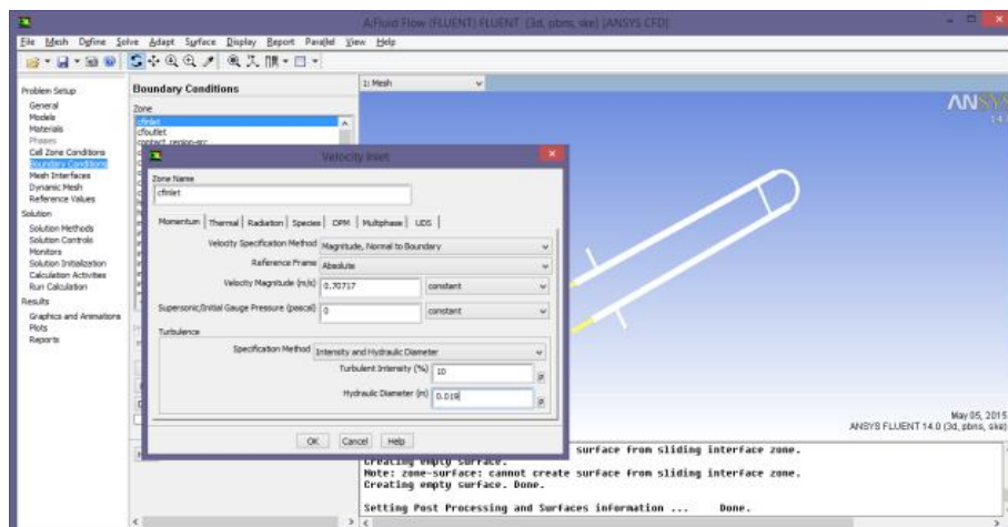
Fig. 2: Boundary conditions given in Problem setup in ANSYS-FLUENT
