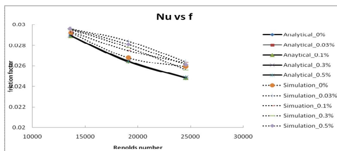
Fig.5: shows that comparison of Numerical friction factor with Blasius correlation for pure water.
