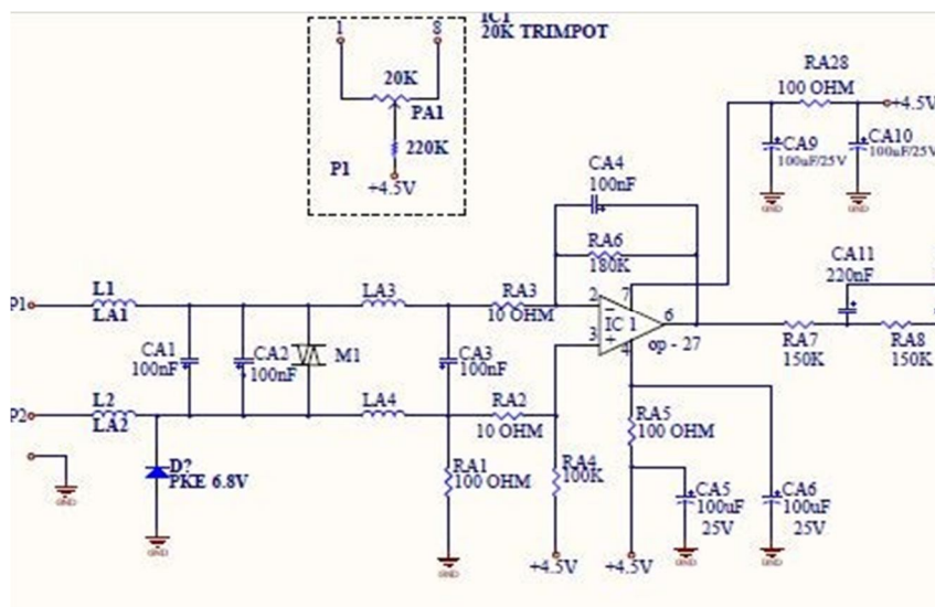
Fig. 6. First Gain Stage
