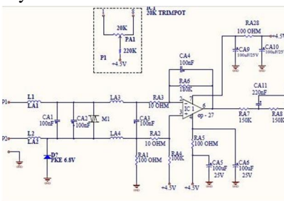
Fig. 4. I to V converter
