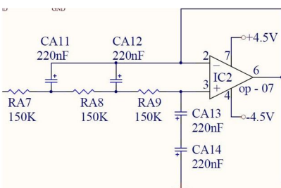
Fig. 5. 3 rd order Sallen-key Low Pass Filter
