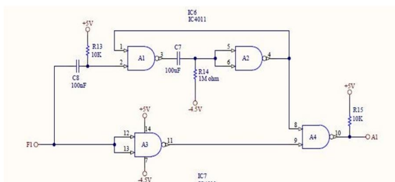
Fig. 3. Digital Filter
