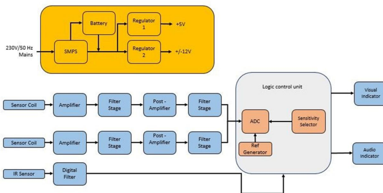
Fig. 1. System Level Block Diagram
