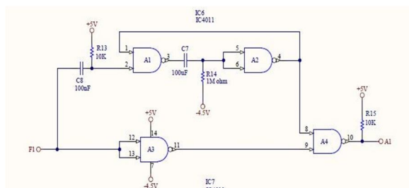
Fig. 3. Digital Filter
