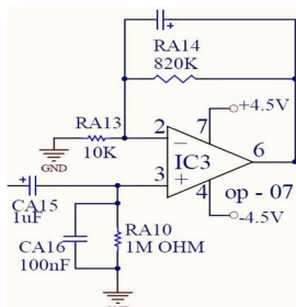
Fig. 7. Second Gain Stage
