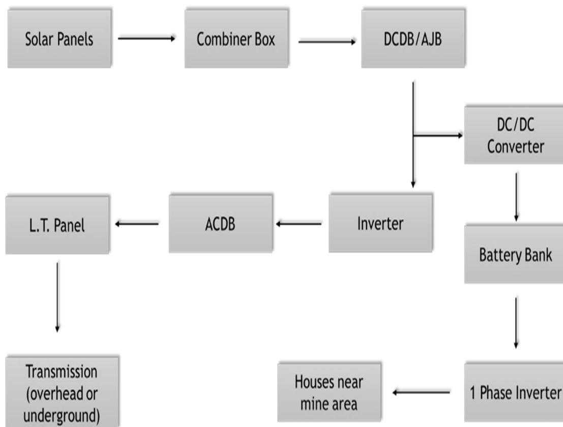
Figure 1: Schematic Diagram of The Plant
