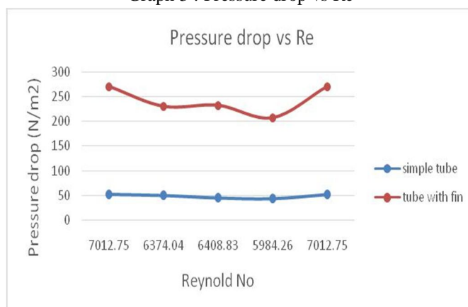
Graph 3 : Pressure drop vs Re
