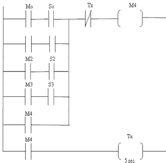
Fig. 4 Ladder Diagram of Stop /Rest Car
