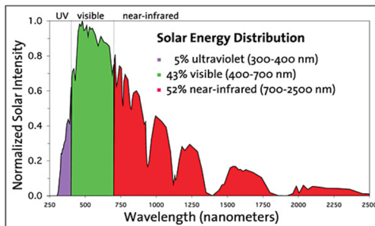
Fig 1: The distribution of solar spectral radiations
