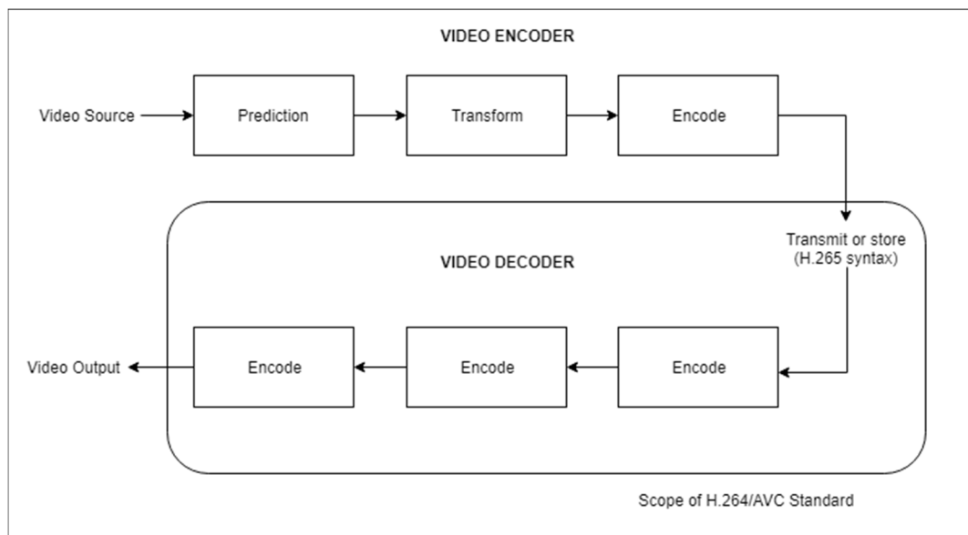
Fig. 1 : Video Encoder and Video Decoder
