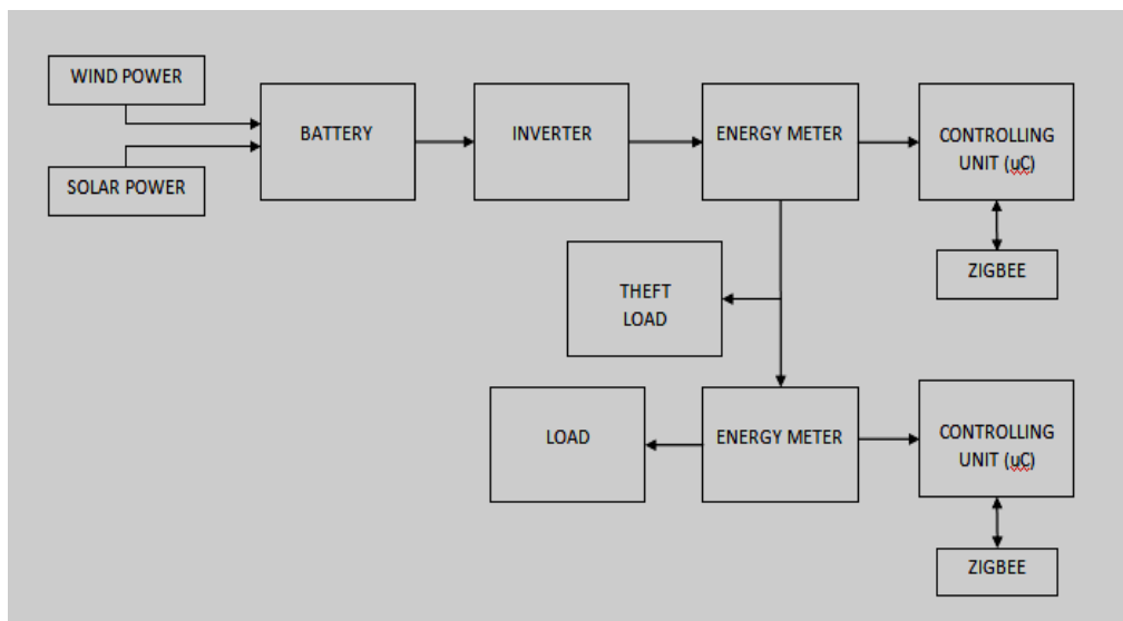
Fig: Proposed system block diagram
