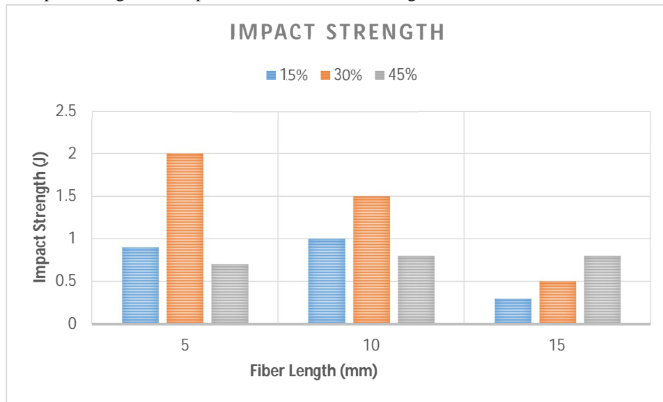
Figure 4.3 Impact Properties of Bamboo Fiber reinforced composites
