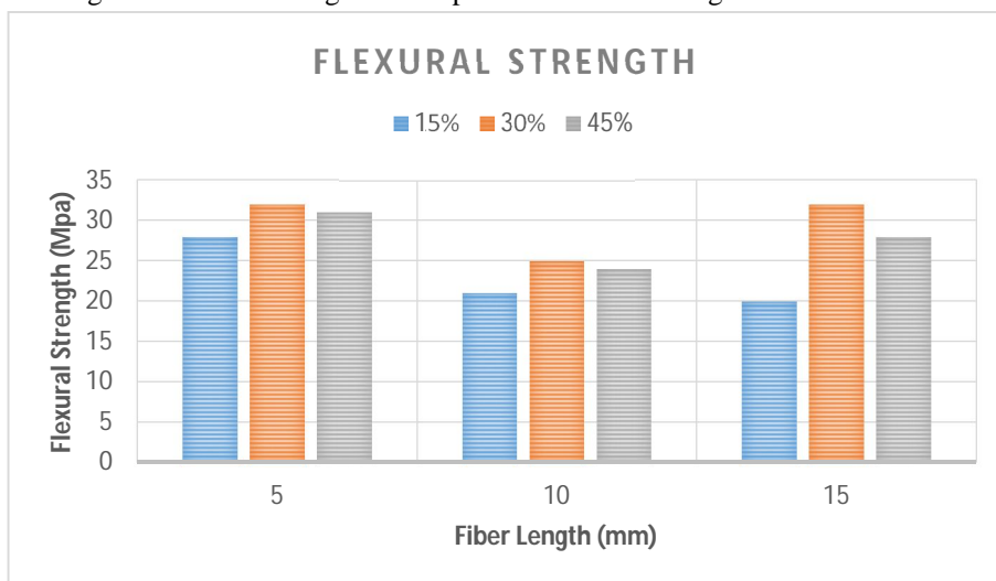
Figure 4.2 Flexural Properties of Bamboo Fiber reinforced composites
