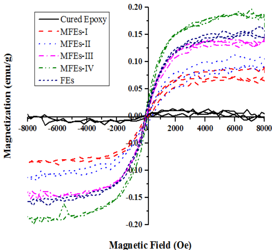
Fig. 2 VSM of different Epoxy-Modified ferrite nanoparticle (MFNEs), Epoxy-Normal ferrite nanoparticles (FNEs) and Cured Epoxy
