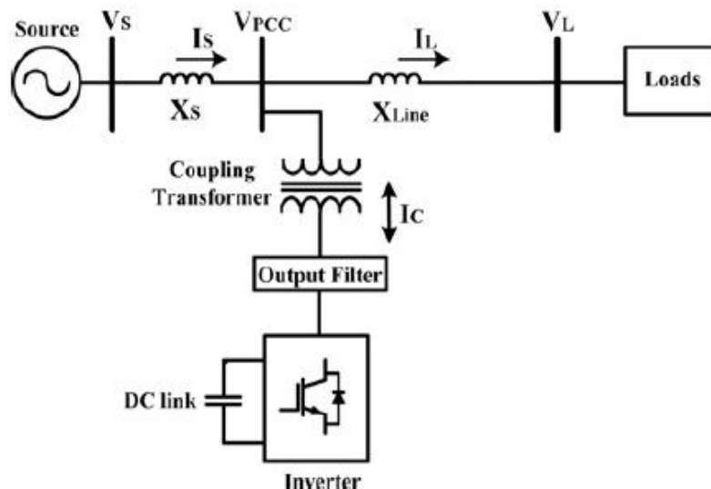
Figure1. Schematic Diagram OF D-STATCOM
