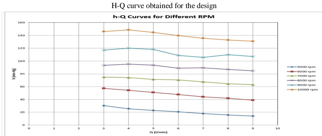
Fig: H-Q curves for optimized design
