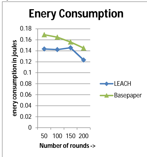
Fig 2: Energy Consumption
