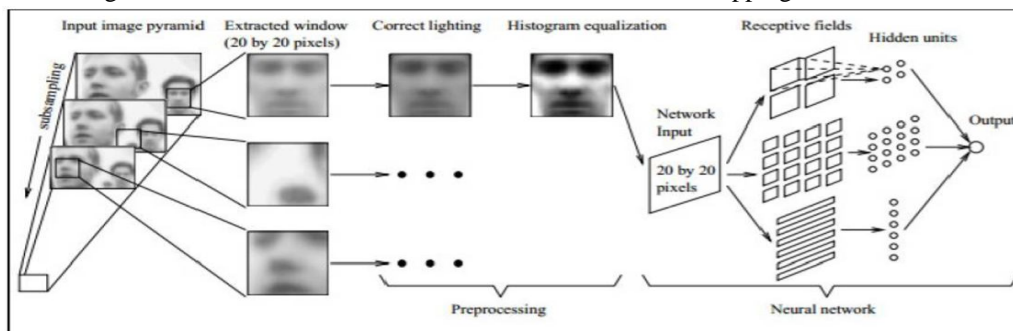
Fig.5. RCNN for face detection[16]
