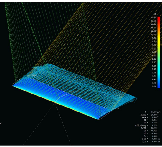
Fig J: XFLR5 model of NACA 0040
