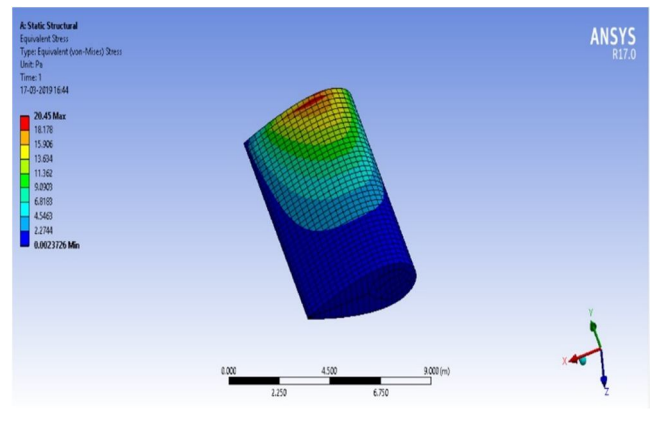
Fig N: Stress distribution of NACA 0030
