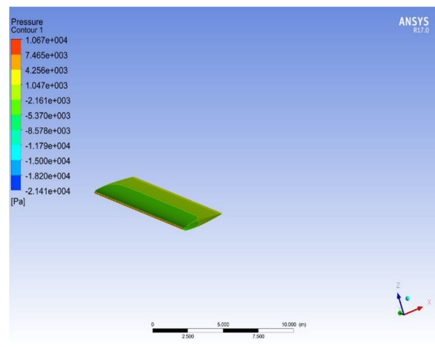
Fig D: Pressure distribution on Wortmann fx63-137
