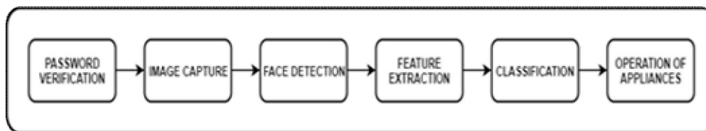
Fig.2.Steps for recognizing images
