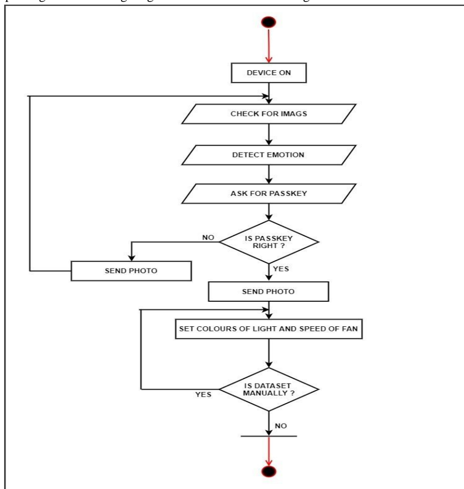
Fig .5 Flowcharts for face recognition system
