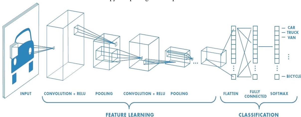
Fig 9. CNN Architecture
