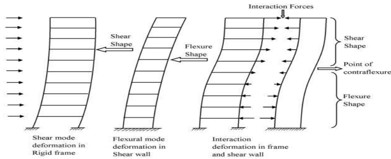
Fig. 1 the Action of Shear Wall-Frame Structure
