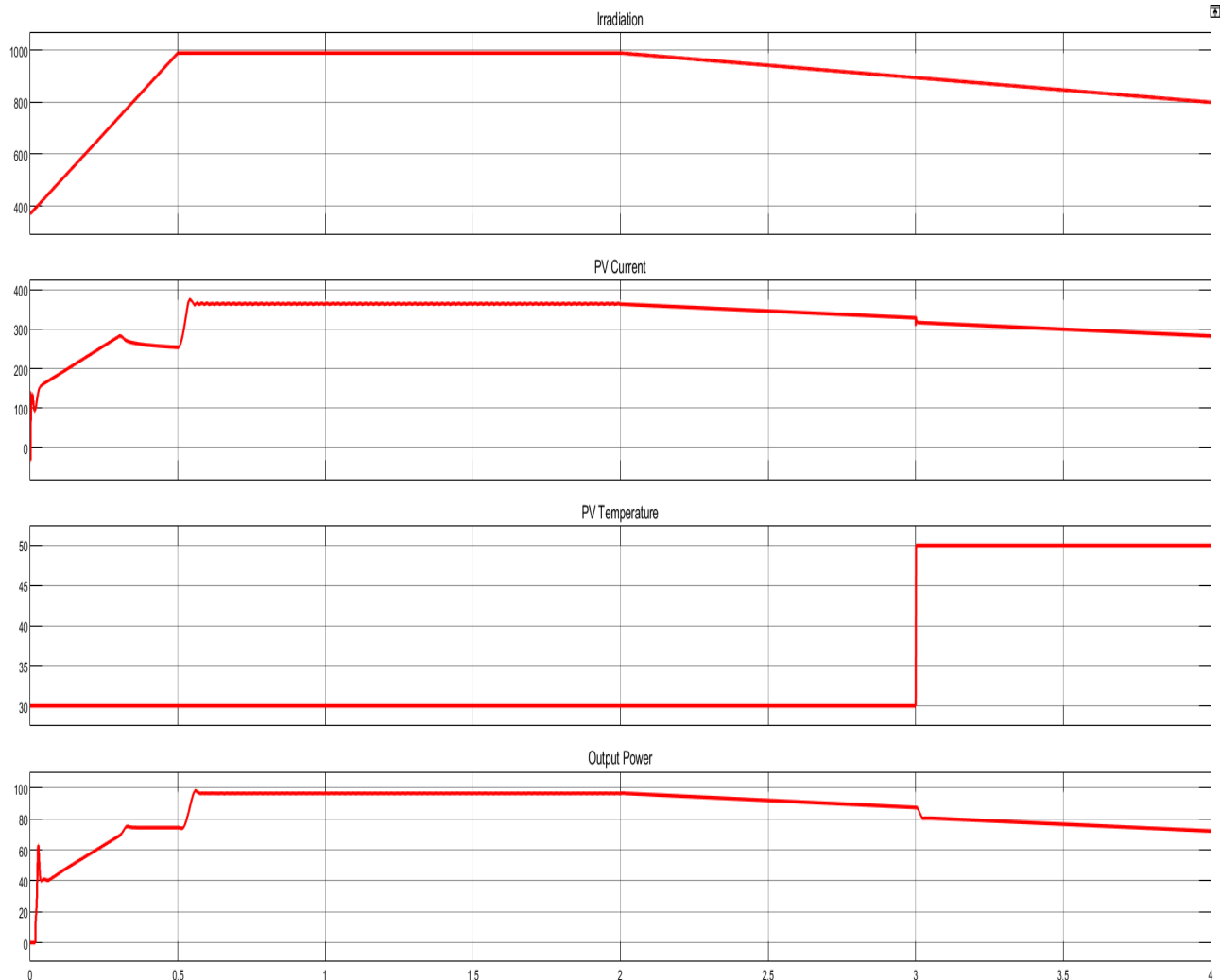
Fig. 8: Simulation results for P & O Algorithm
