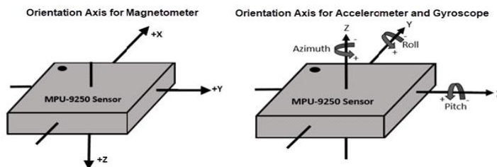
Fig. 3. MPU-9250 Orientation
