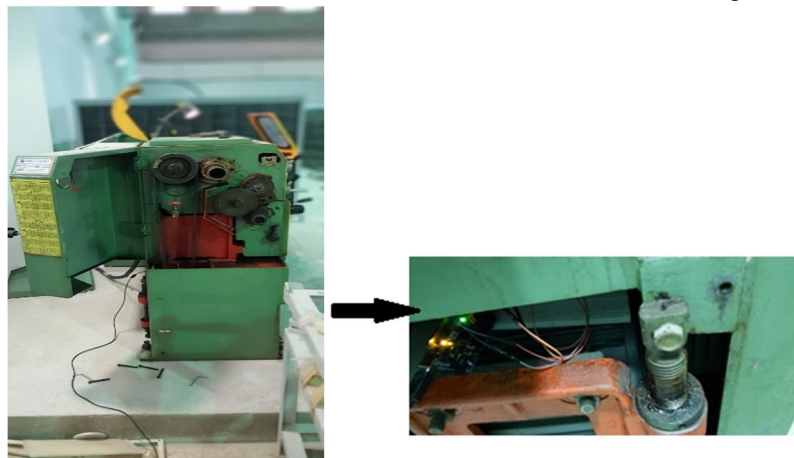
(a): Side view for lathe machine (b): fixation of present work Arduino package. Fig. 8. Inside view of lathe machine
