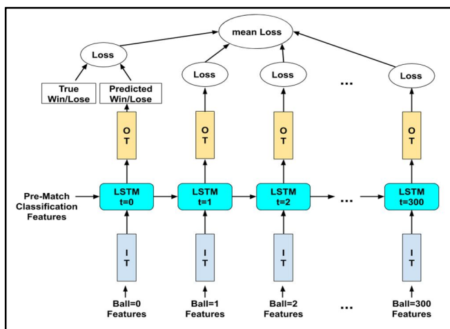
Fig. 2b Our All inputs all outputs model.
