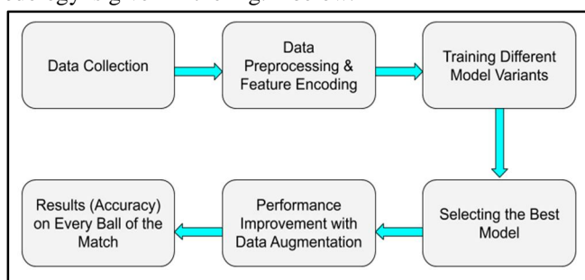
Fig. 1 Workflow Diagram
