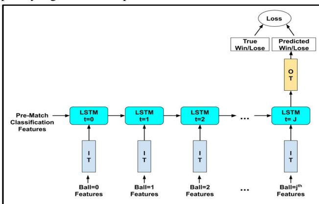
Fig. 2a Our all inputs single output model.
