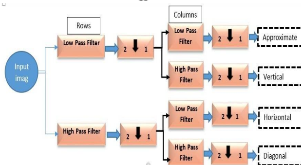
Fig. 3. Diagram of Discrete Wavelet Transform (DWT)
