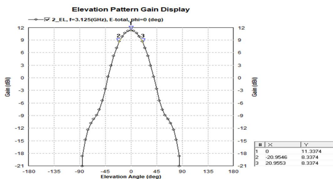
Figure 5: Radiation pattern for PHI=0°
