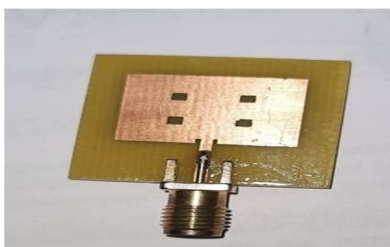
Figure 2: Hardware of Metamaterials Patch Antenna
