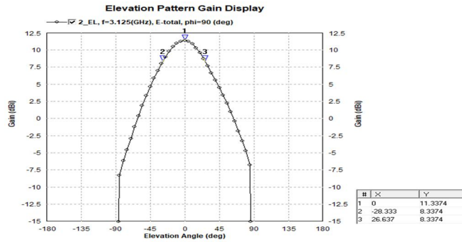
Figure 6: Radiation Pattern FOR PHI=90 0
