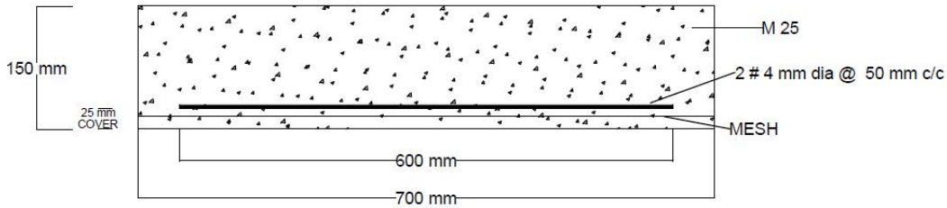
TYPE II : M25 REINFORCED BEAM WITH MESH
