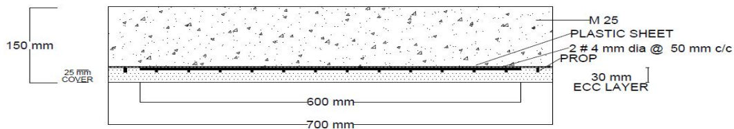
TYPE IX : ECC-RCC UNBOUND + PROPPED COMPOSITE BEAM
