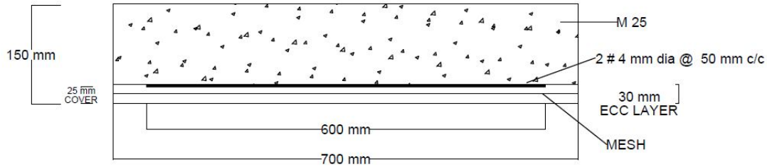
TYPE VI : ECC-RCC BONDED COMPOSITE BEAM WITH MESH
