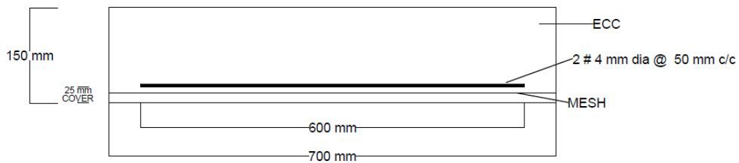
TYPE IV : ECC REINFORCED BEAM WITH MESH
