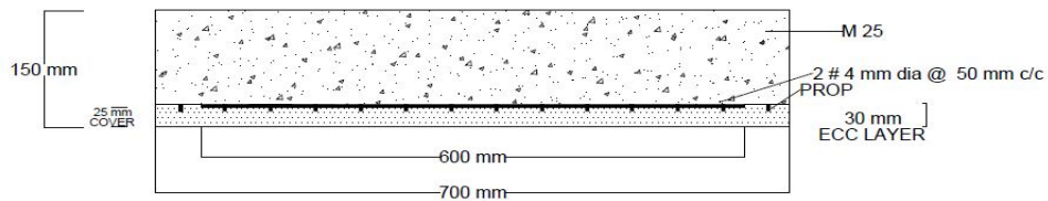
TYPE VII : ECC-RCC BONDED + PROPPED COMPOSITE BEAM
