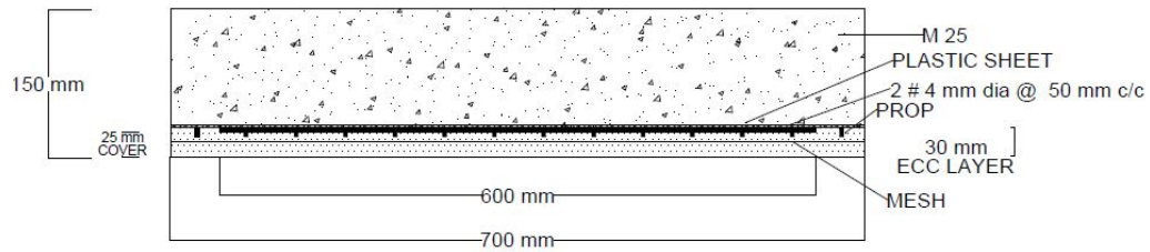
TYPE X : ECC-RCC UNBOUND + PROPPED COMPOSITE BEAM WITH MESH
