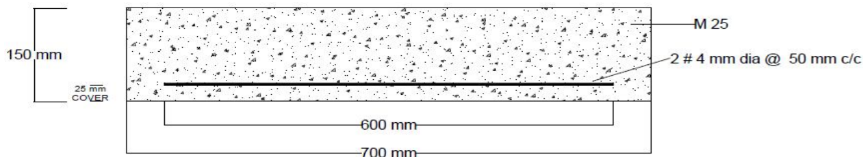
TYPE I : M25 REINFORCED BEAM
