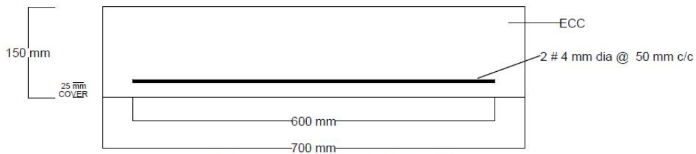
TYPE III : ECC REINFORCED BEAM
