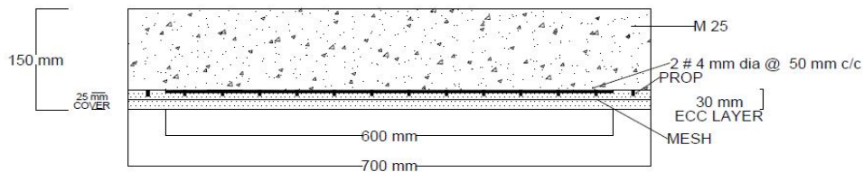
TYPE VIII : ECC-RCC BONDED + PROPPED COMPOSITE BEAM WITH MESH
