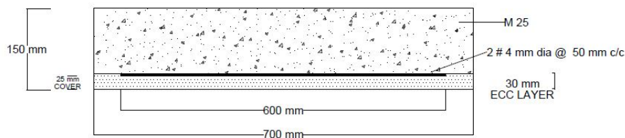
TYPE V : ECC-RCC BONDED COMPOSITE BEAM
