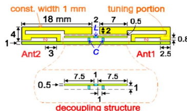
Figure 1 (b): Side view of the antenna part and feeding part
