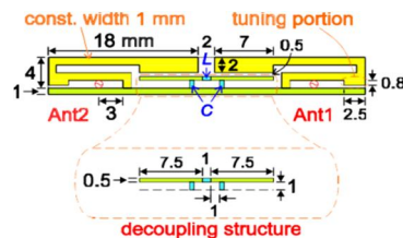
Figure 1 (b): Side view of the antenna part and feeding part
