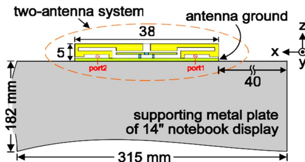
Figure 1 (a): Top view of Existing f shaped patch antenna
