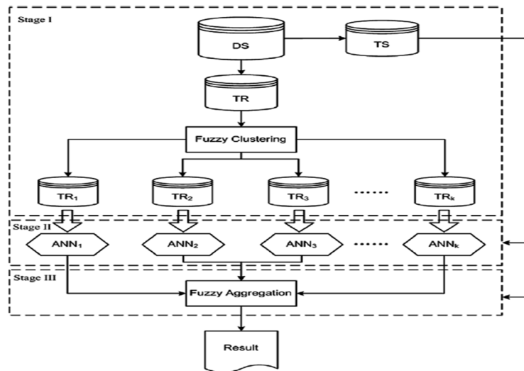
Figure 2: Framework of FC-ANN for IDS
