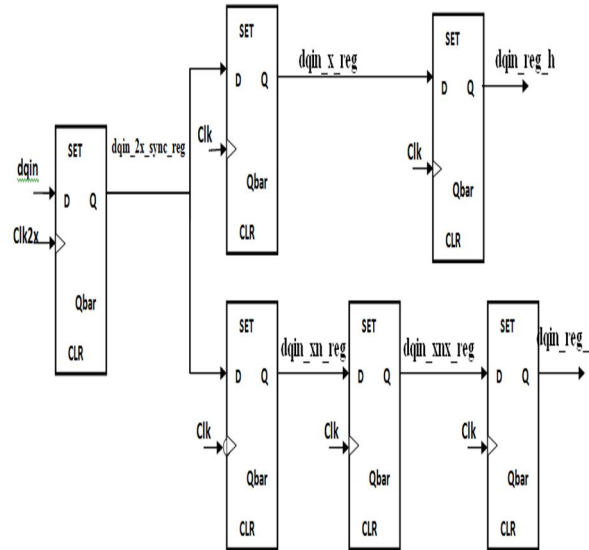
Fig.5. Read data path for DDR SDRAM Controller.
