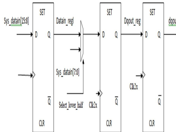
Fig.6. Write data path for DDR SDRAM Controller
