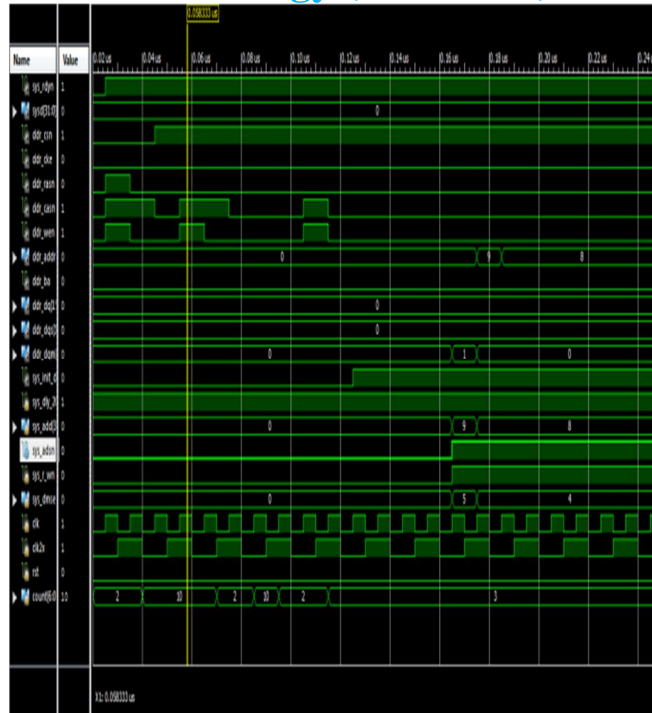
Fig.7. Simulation results of DDR SDRAM controller
