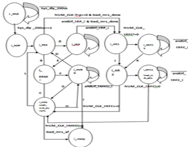
Fig.3. DDR SDRAM Initialization FSM (INIT_FSM) state diagram .
