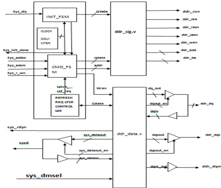
Fig.2. Functional block diagram of DDR SDRAM controller .
