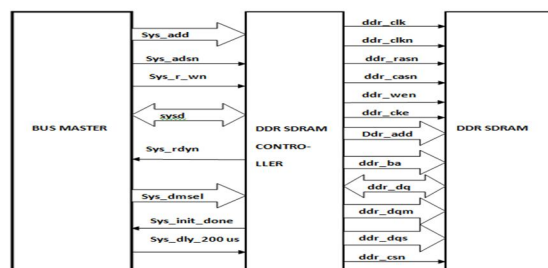
Fig. 1. DDR SDRAM controller system
