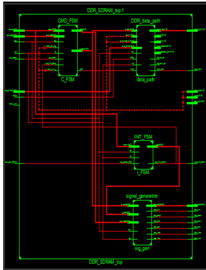
Fig.8. RTL Schematic of DDR SDRAM
