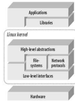
Figure.1: Linux OS Architecture
