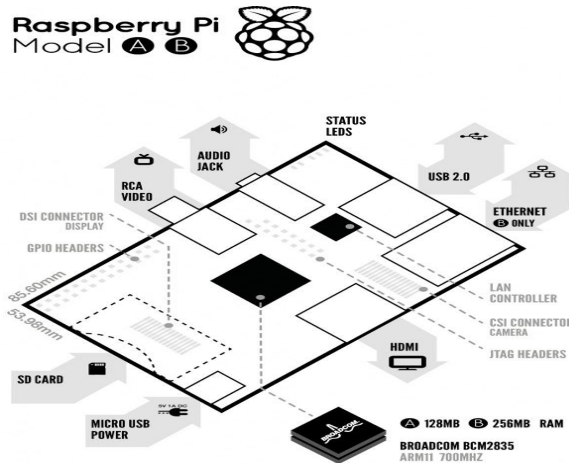
Figure.3: Board Features
