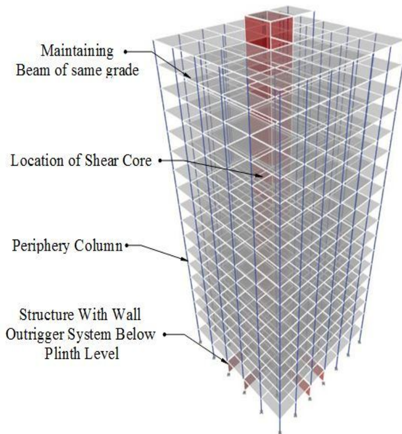
Fig. 2: Structure with Dual Structure Configuration with Wall Outrigger System below Plinth Level
