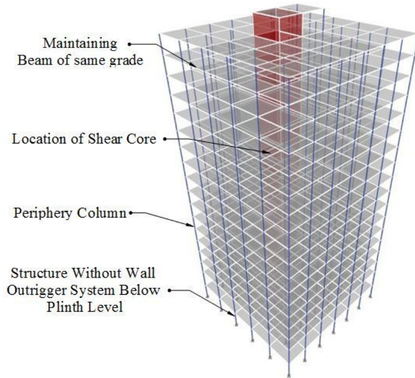
Fig. 1: Structure with Dual Structure Configuration without Wall Outrigger System
