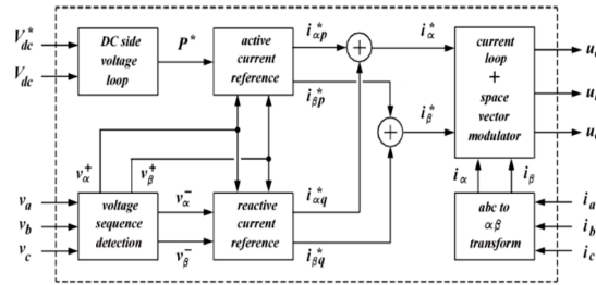
Fig. 2. Diagram of the STATCOM control system.
