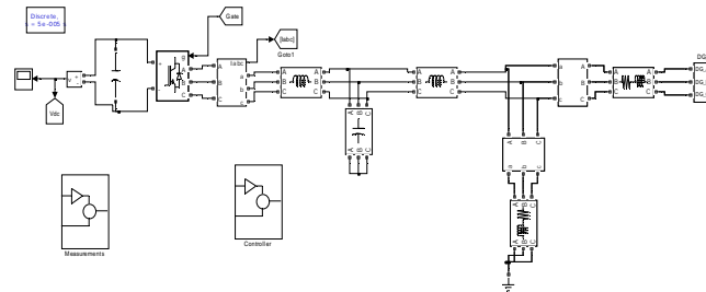
Fig.9. Simulation model for proposed circuit
