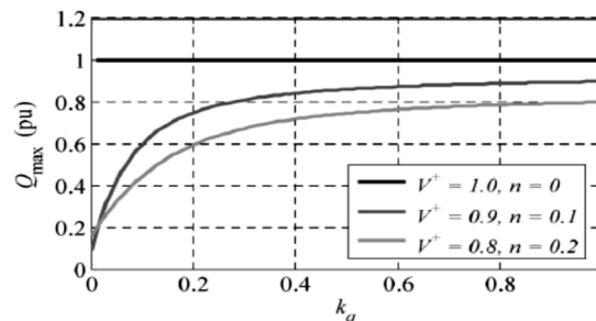
Fig. 3. Maximum reactive power versus control gain k_q and for several values of V^+ and n ( I_{\max} = 1 p.u., \cos_{\min} = -0.5 ), defined as the higher phase current amplitude, and from (21), it can be written as
