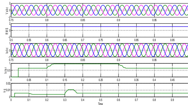
Fig.8. Simulation results of STATCOM When K_q=1 - PCC Voltage ( V_{abc} ), RMS voltage ( V_{RMS} ), Current ( I_{abc} ), I^* and K_q .
