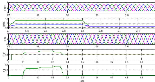
Fig.10. Simulation results of STATCOM when K_q=0.5 – PCC Voltage ( V_{abc} ), RMS voltage ( V_{RMS} ), Current ( I_{abc} ), I^* and K_q .
