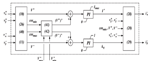
Fig. 4. Diagram of the proposed reactive current reference generator with voltage support auxiliary service.
