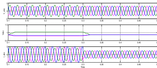
Fig.6. Simulation results of STATCOM operation in steady state and under the voltage- PCC Voltage ( V_{abc} ), RMS voltage ( V_{RMS} ), Current ( I_{abc} ), I^* and K_q .
