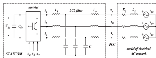
Fig. 1. Diagram of the power system, including the STATCOM and the model of the electrical ac network.
