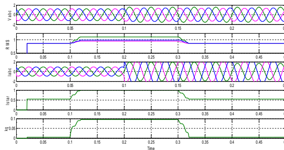
Fig.12. Simulation results when STATCOM is in active_ PCC Voltage ( V_{abc} ), RMS voltage ( V_{RMS} ) and current ( I_{abc} ) I^* and K_q .
