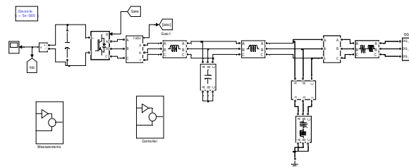
Fig.11. Simulation model for proposed circuit
