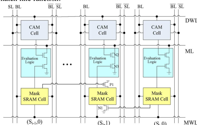
Fig. 3 Two-Side Self-Gating Ternary CAM array
