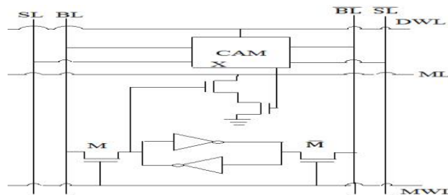
Fig.5 Schematic of a 4T-Ternary CAM cell
