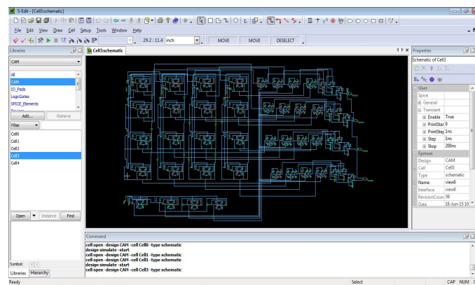
Fig. 9 Schematic entries of 4x4 TCAM cells with MLSA
