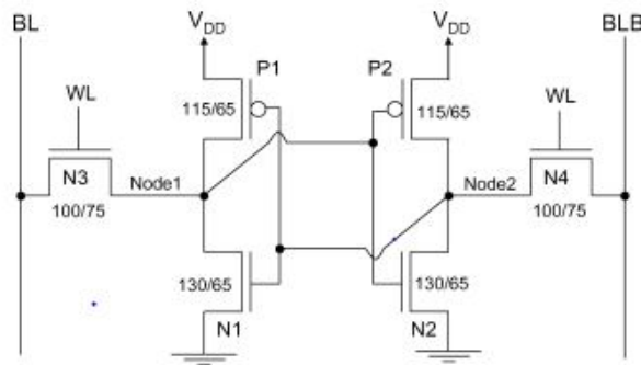
Fig. 4 Proposed circuit of 6T based SRAM
