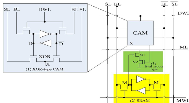
Fig. 2 XOR type Single CAM cell
