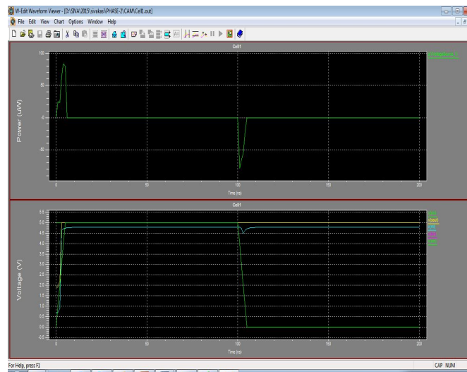
Fig.11 Power consumption of 4x4TCAM cell (4T based)
