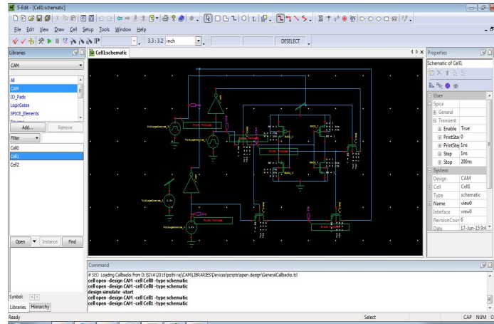
Fig. 7 Schematic entry of 8T based Ternary CAM design
