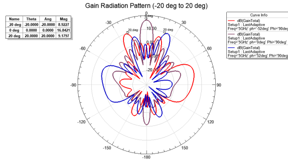
Figure 23: Gain Radiation Pattern of 2x8 CP Phased Array
