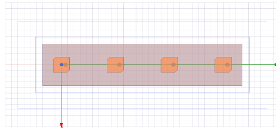
Figure 15: Design of 1x4 CP Phased Array Antenna
