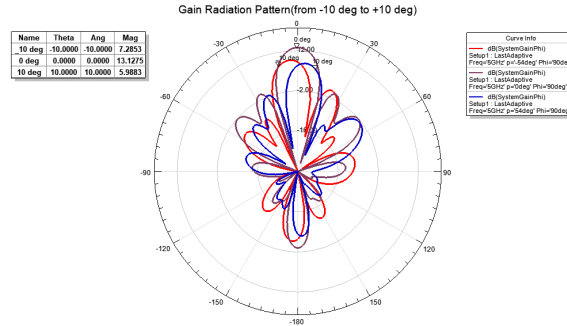
Figure 12: Gain Radiation Pattern of four 1x2 LP Phased Array
