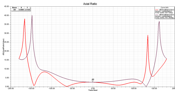
Figure 7: Axial Ratio of CP Single Patch Antenna
