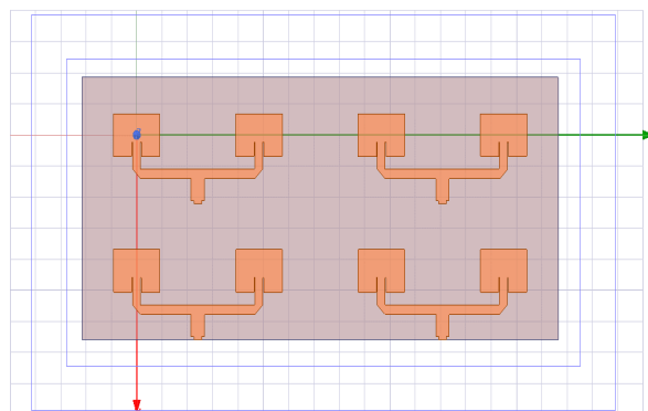
Figure 11: Design of four 1x2 LP Phased Array Antenna
