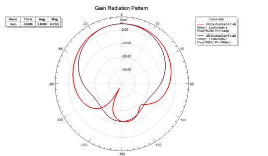
Figure 4: Gain Radiation Pattern of LP Single Patch Antenna
