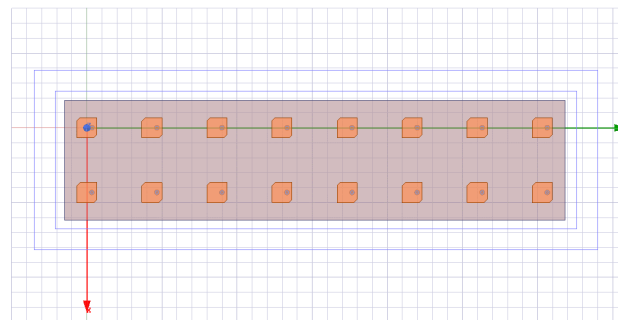
Figure 21: Design of 2x8 CP Phased Array Antenna
