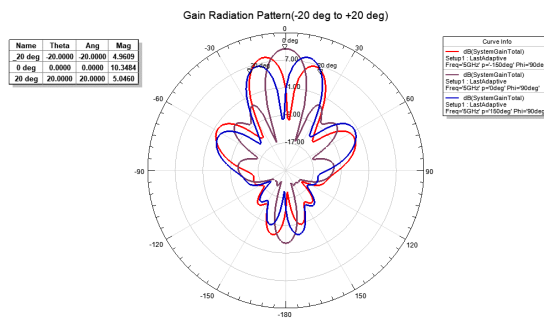
Figure 10: Gain Radiation Pattern of two 1x2 LP Phased Array
