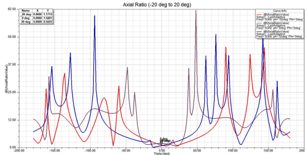
Figure 19: Axial Ratio of 1x4 CP Phased Array Antenna
