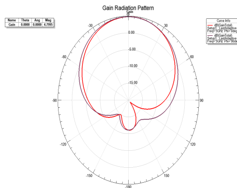
Figure 8: Gain Radiation Pattern of CP Single Patch Antenna
