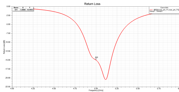
Figure 6: Return Loss of CP Single Patch Antenna
