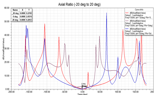
Figure 22: Axial Ratio of 2x8 CP Phased Array Antenna
