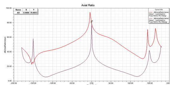
Figure 3: Axial Ratio of LP Single Patch Antenna
