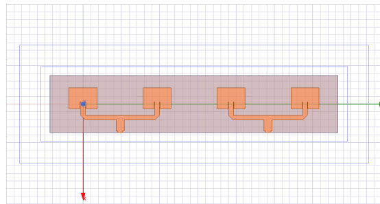
Figure 9: Design of two 1x2 LP Phased Array Antenna
