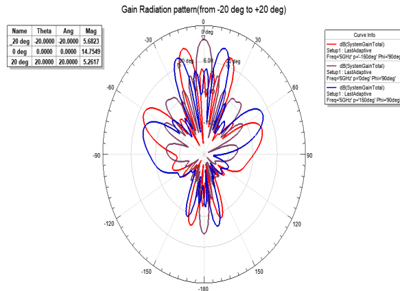
Figure 14: Gain Radiation Pattern of four 2x2 LP Phased Array
