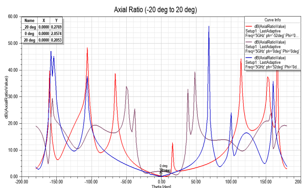
Figure 22: Axial Ratio of 2x8 CP Phased Array Antenna
