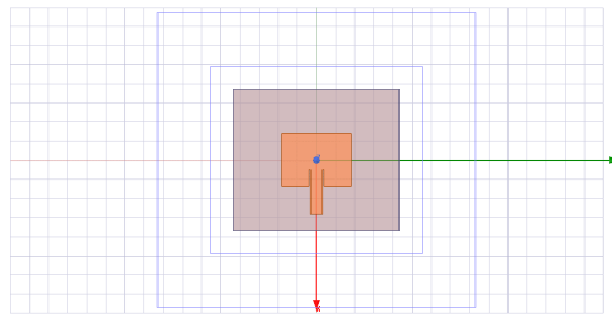
Figure 1: Design of LP Single Patch Antenna
