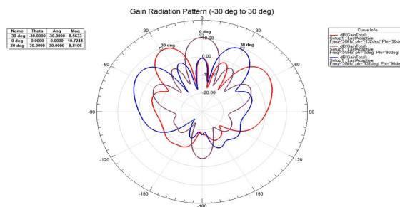
Figure 17: Gain Radiation Pattern of 1x4 CP Phased Array
