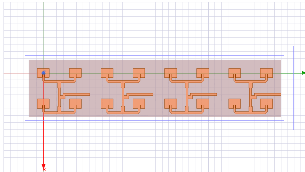
Figure 13: Design of four 2x2 LP Phased Array Antenna
