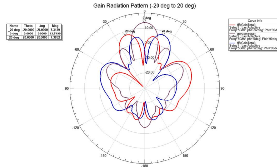
Figure 20: Gain Radiation Pattern of 2x4 CP Phased Array
