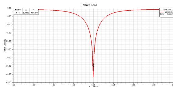
Figure 2: Return Loss of LP Single Patch Antenna
