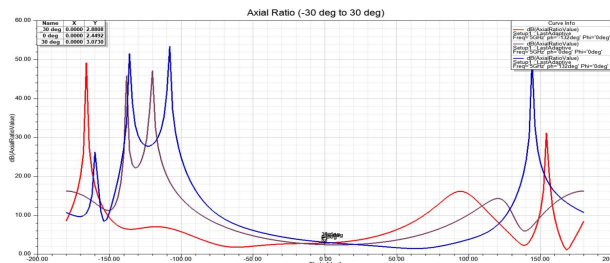
Figure 16: Axial Ratio of 1x4 CP Phased Array Antenna
