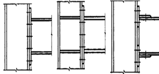
Figure 1.2. Various types of rigid connections (a) End plate without column stiffener (b) End plate with column stiffener (c) T-Stub connection (Subramanium 2007)
