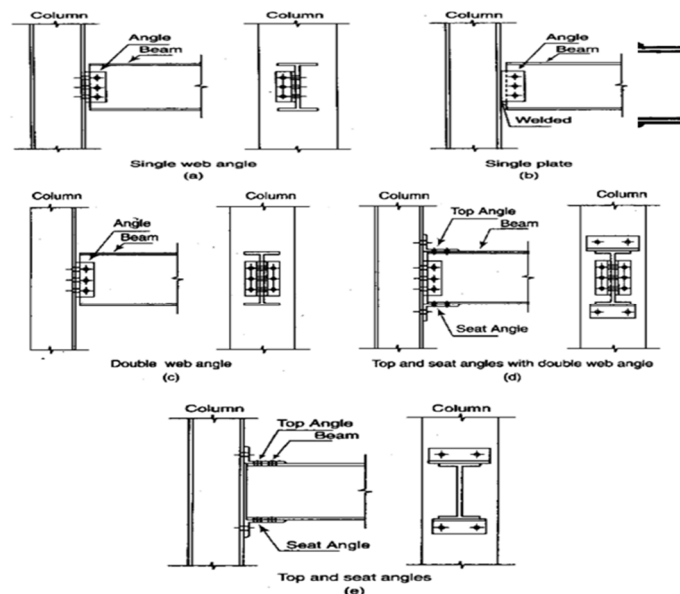
Figure 1.3. Various types of Semi- rigid connections (a) Single web angle (b) Single plate (c) Double web angle (d) Top and Seat angle with Double web angle (e) Top and seat angles (Subramanium 2007)
