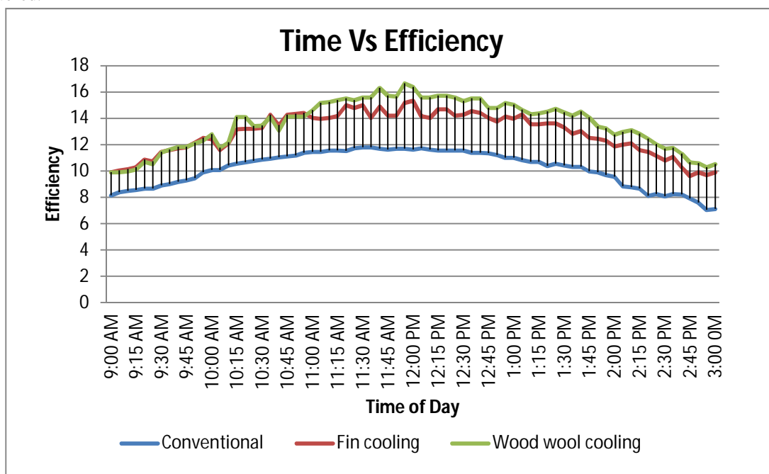
Fig. 10 A comparison between efficiency of modified system & conventional system
