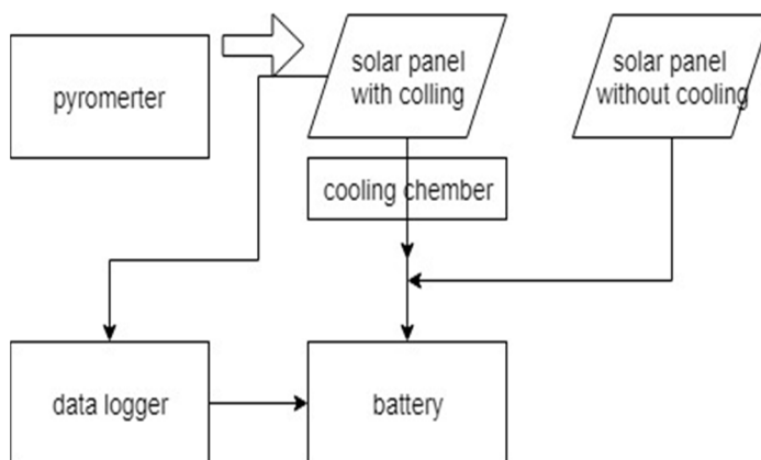
Fig:4 Block diagram of experimental set up of photovoltaic panels
