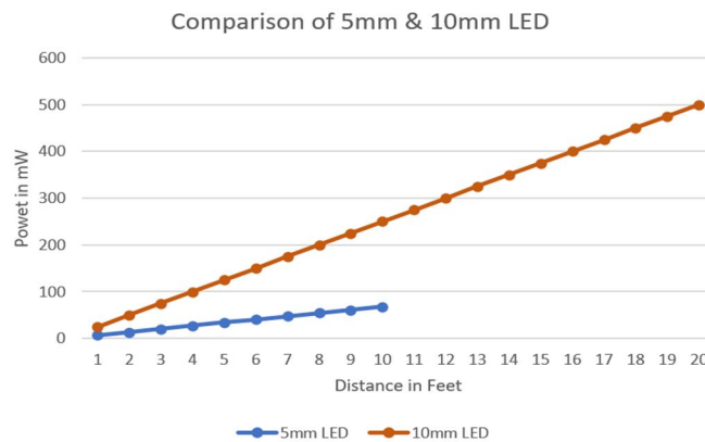
Fig. 9: Comparison of 5mm & 10mm LED used for data transmission
