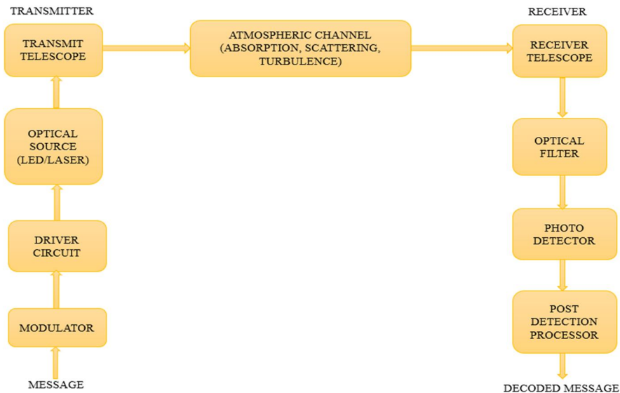
Fig. 3: Block diagram of FSO system
