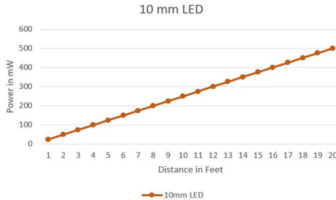
Fig. 8: 10mm LED used for data transmission
