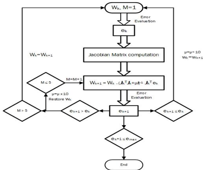
Fig.4 Flow diagram of LM Algorithm
