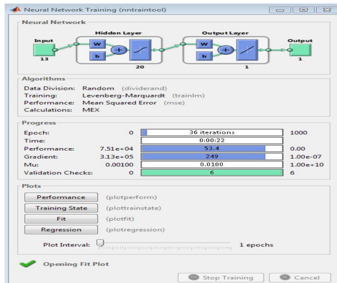
Fig.5 Designed ANN Structure
