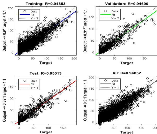
Fig.8 Regression Analysis of proposed system
