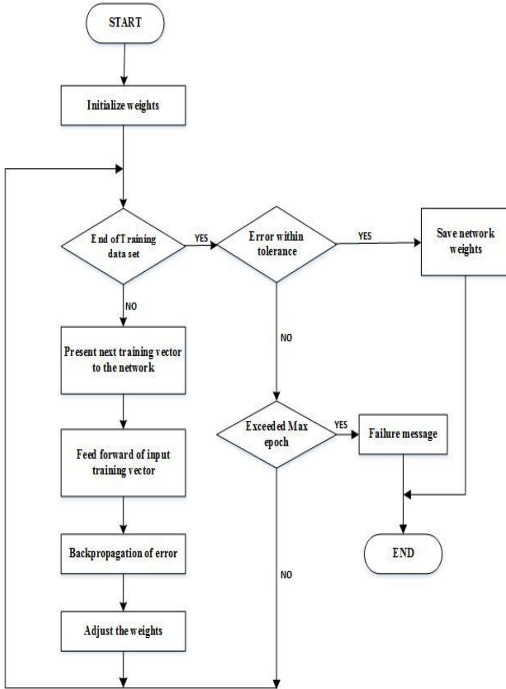
Fig.3 Flowchart of Back Propagation
