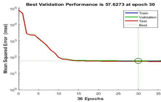
Fig.7 Reduction of MSE with respect to epochs
