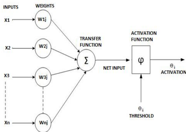
Fig.2 Mathematical Modeling of ANN
