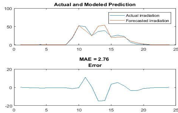
Fig.6 Predicted and Actual Solar Irradiation
