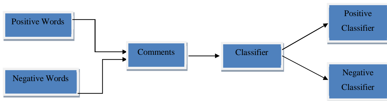
Fig. Algorithm Of Naive Bayes P(\mathbf{X} = \mathbf{x} | C = c) P(C = c)
