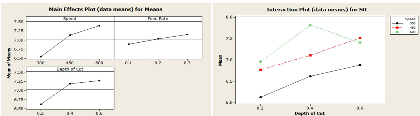
Fig. 4: (a) Main effect plot for Surface Roughness; (b) Interaction plot for Surface Roughness with parameters
