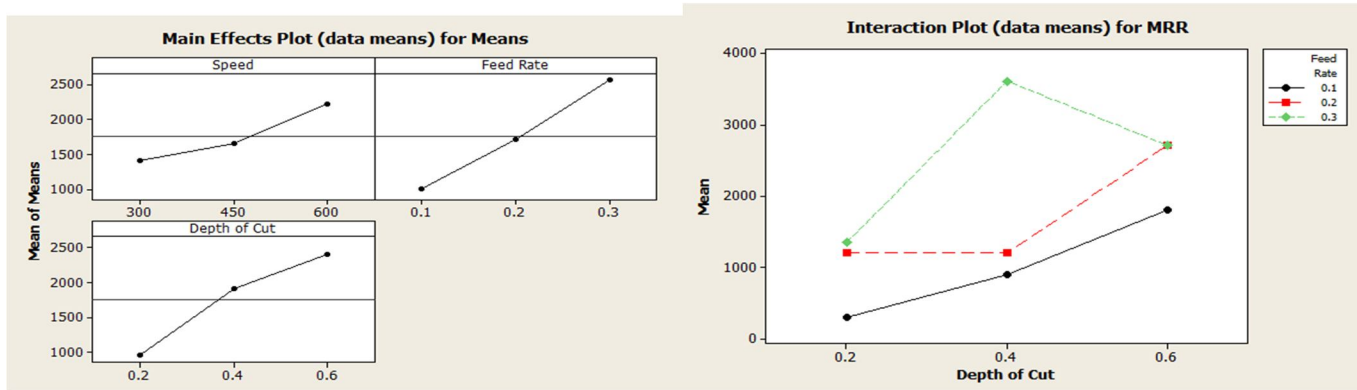
Fig. 3: (a) Main effect plot for MRR; (b) Interaction plot for MRR with parameters
