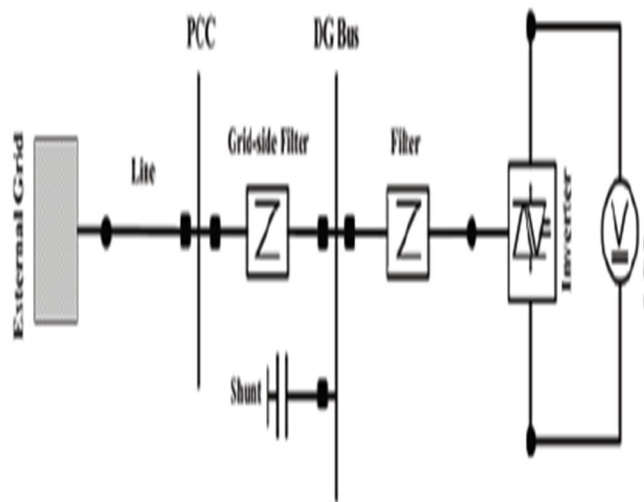
Fig .7 Power stage of the three-phase DG unit (single line Presentation)
