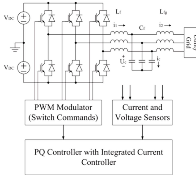
Fig.1 Structure of a three phase VSI used for a DG system.
