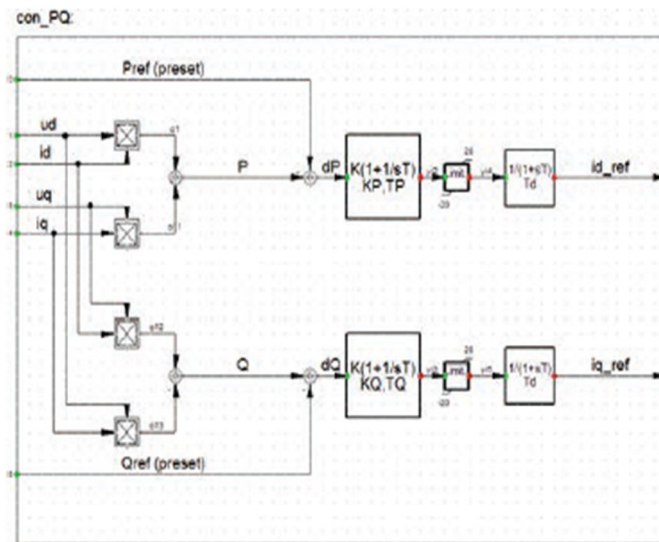
Fig 10 PQ control block
