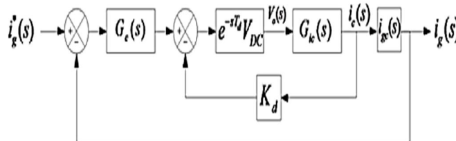
Fig.4 Dual loop regulator with capacitor current active damping.
