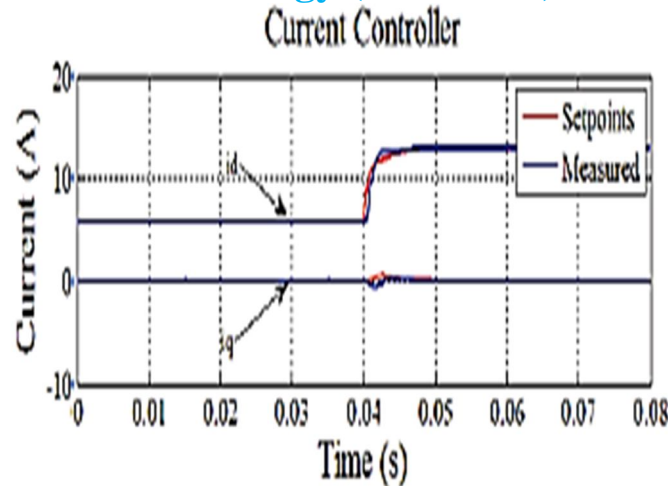
Fig 14 grid currents and injected power to grid current controller wave forms
