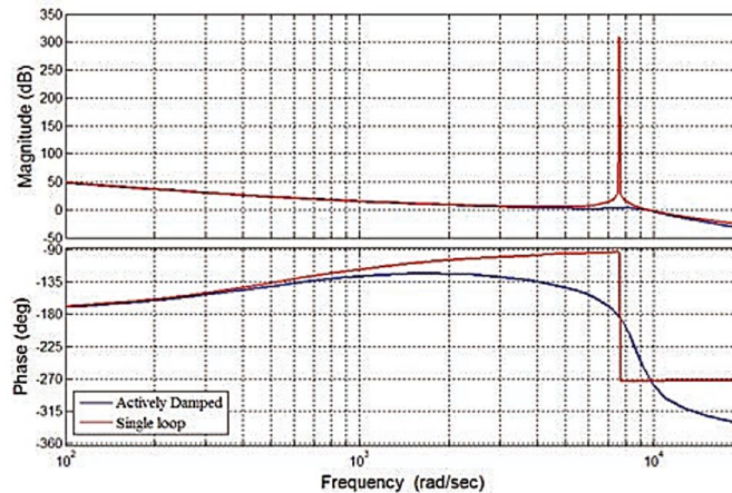
Fig. 5 Bode plot of the transfer function as defined in (8) and (9).
