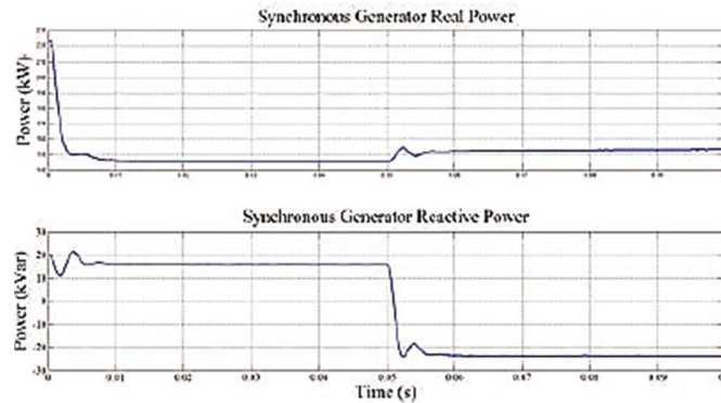
Fig. 16 synchronous generator powers
