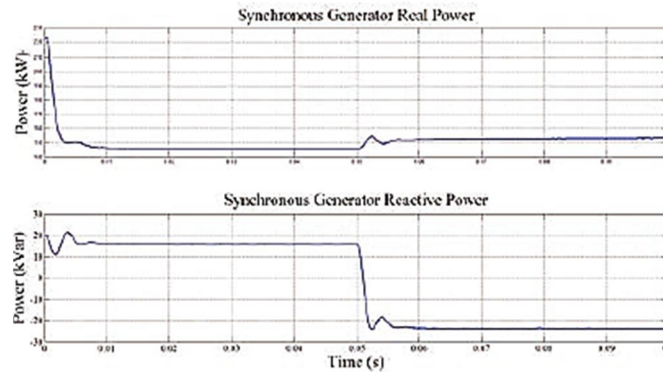
Fig. 16 synchronous generator powers
