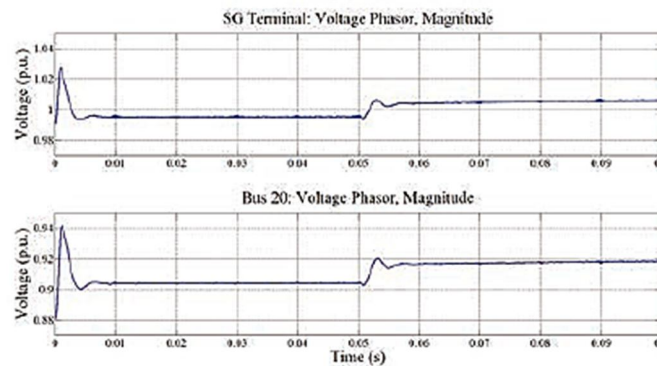
Fig 17 voltage profile along the feeder
