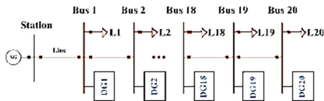
Fig 15 20 bus micro grid
