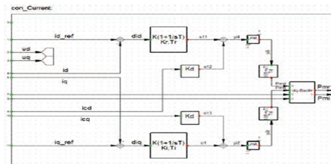
Fig 9 current control block
