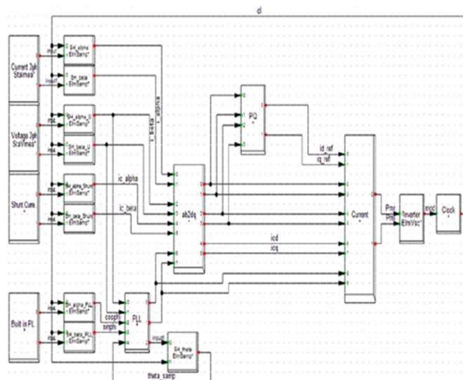
Fig. 11 DG converter controller implemented in DigSILENT
