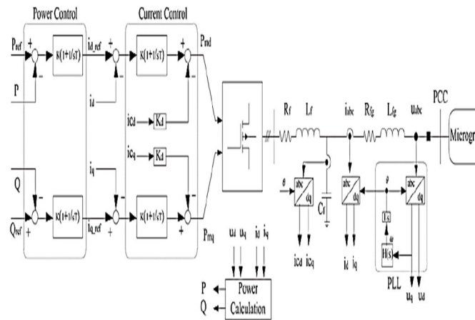
Fig. 2 Schematic diagram of the three-phase DG unit and its corresponding control architecture.
