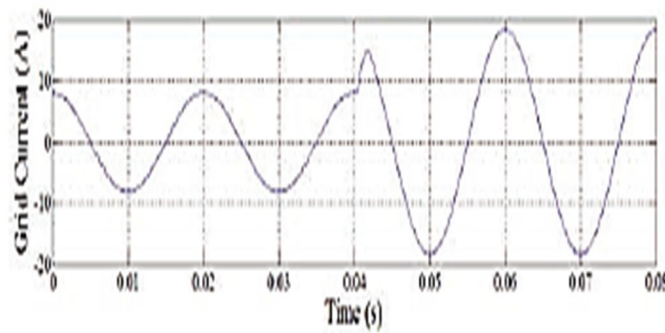
Fig 13 Phase A Current with step change in Power Reference Grid side.
