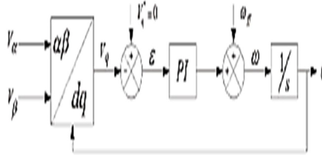
Fig .6 .Three-phase dq-PLL.
