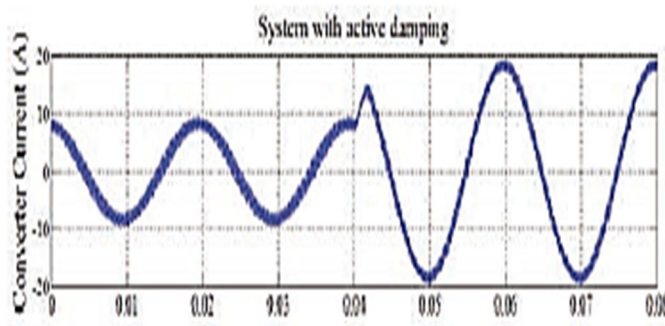
Fig.12 Phase A Current with step change in Power Reference Converter side
