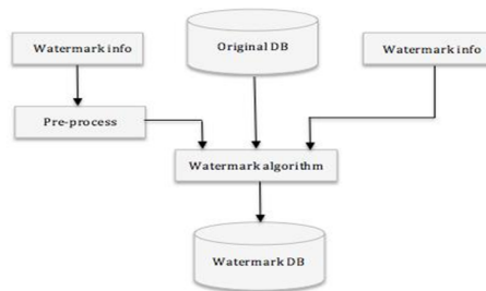
Figure 1 Model of relational database watermarking embedding
