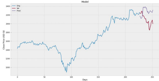
Fig. 2b Reliance NS Polynomial Kernel Prediction
