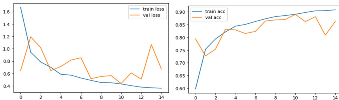
Fig 4. Plot of accuracy and loss against epoch(VGG19)
