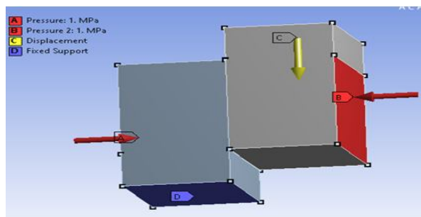
Fig. 6 Loading and Boundary Condition at Joint
