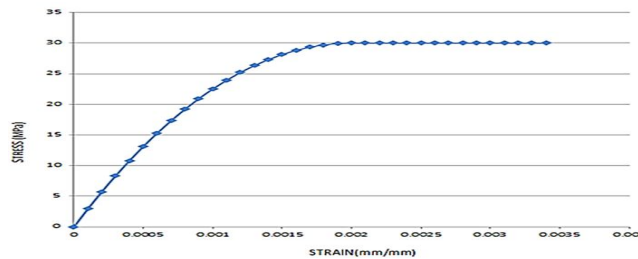
Fig. 4 Stress Strain Curve of Concrete
