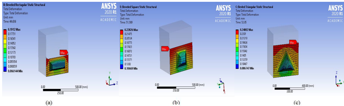
Fig. 12 Total Deformation in keyed region of (a) Bevelled Rectangle Key Dry Joint (b) Bevelled Square Key Dry Joint (c) Bevelled Triangular Key Dry Joint
