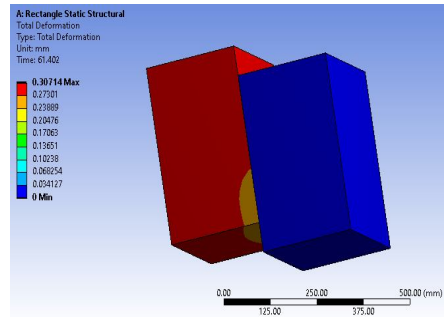
Fig. 11 Typical Total Deformation in Dry Joint
