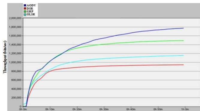
Figure 2. Throughput comparison in four routing protocols
