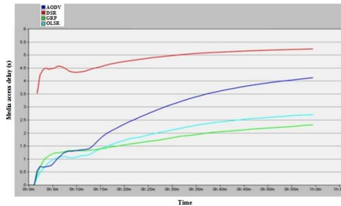
Figure 4. Media access delay comparison in four routing protocols
