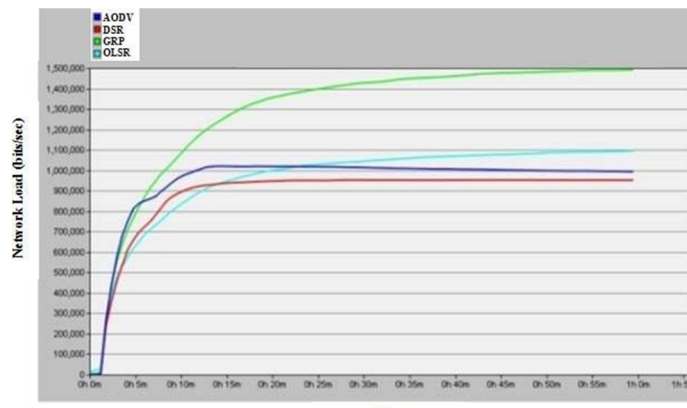
Figure 3. Network load comparison in four routing protocols
