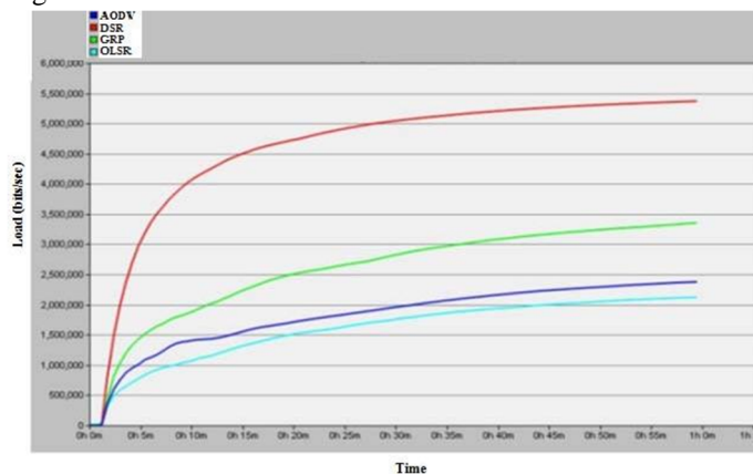
Figure 5. Load (bits/sec) comparison in four routing protocols
