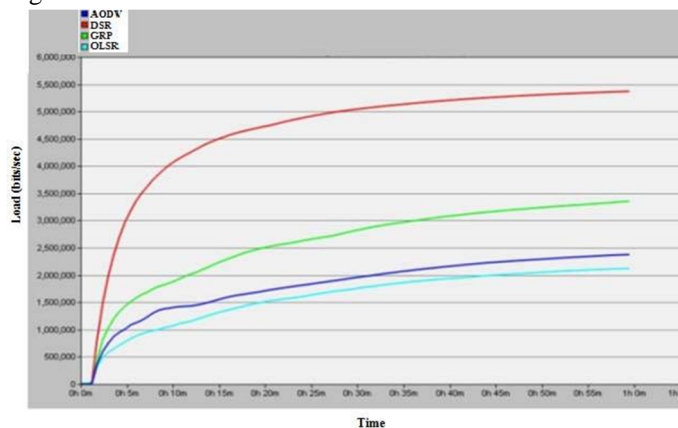
Figure 5. Load (bits/sec) comparison in four routing protocols
