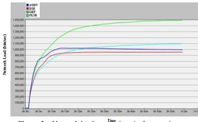
Figure 3. Network load comparison in four routing protocols
