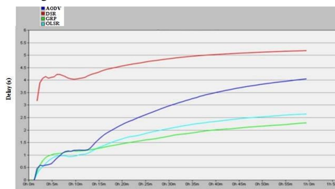
Figure 6. Delay (s) comparison in four routing protocols
