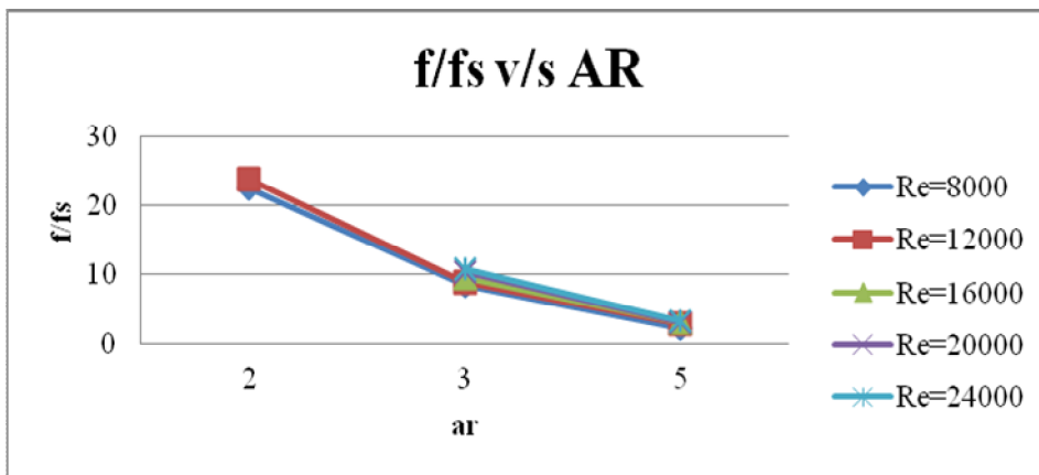
Fig.11: Variation of f/fs with AR (p=8mm), Detachment=4mm
