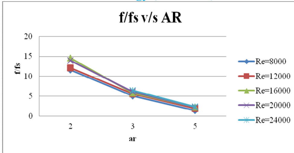
Fig 13: Variation of f/fs on AR ( p=16mm ), Detachment=4mm
