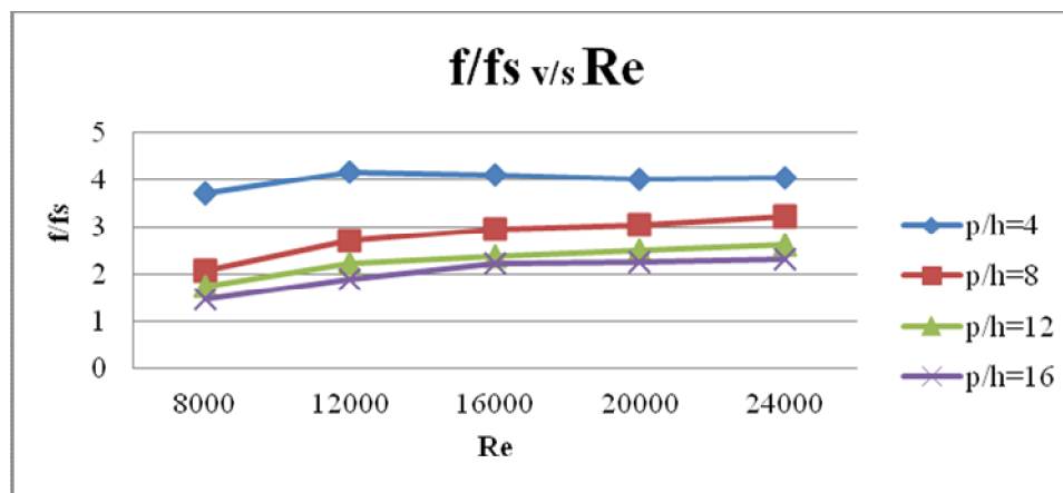
Fig 7: Variation of f/fs with Re (AR=2, h=6mm), Detachment=4mm
