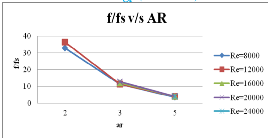
Fig 10: Variation of f/fs with AR (p=4mm), Detachment=4mm
