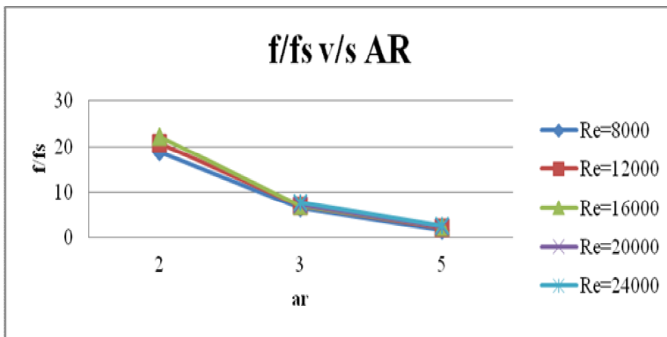
Fig 12: Variation of f/fs on AR (p = 12mm), Detachment=4mm
