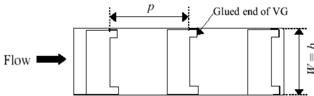
Fig. 3: Arrangement of detached ribs
