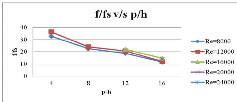
Fig 6: Variation of f/fs with p/h (AR=5, h=15mm), Detachment=4mm
