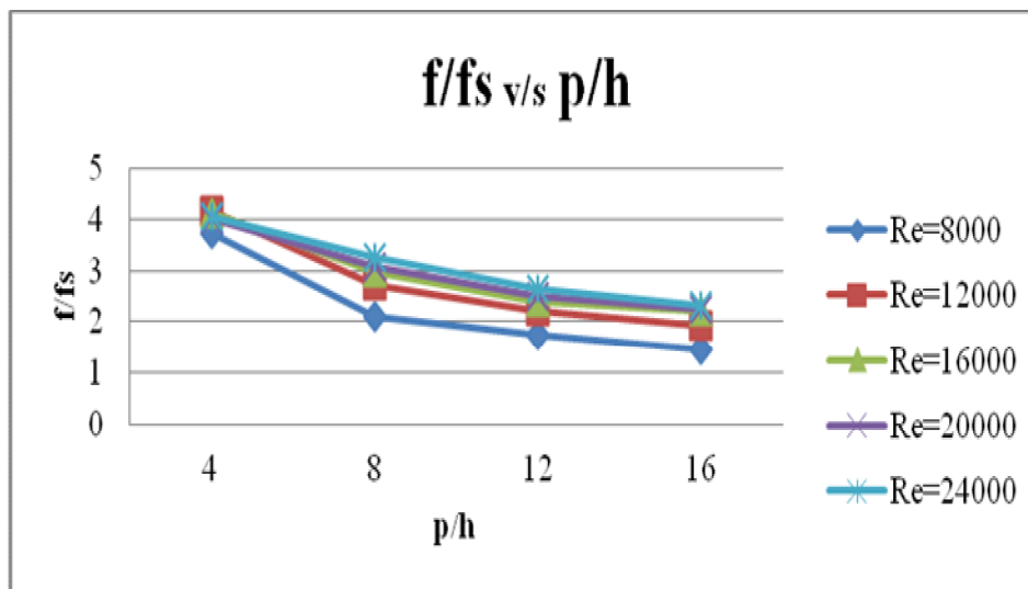
Fig. 4: variation of f/fs with p/h (AR=2, h=6mm), Detachment=4mm
