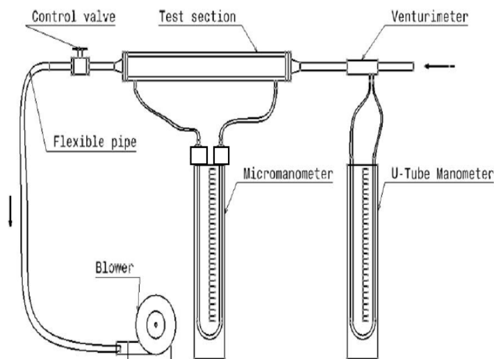
Fig. 1: Experimental setup
