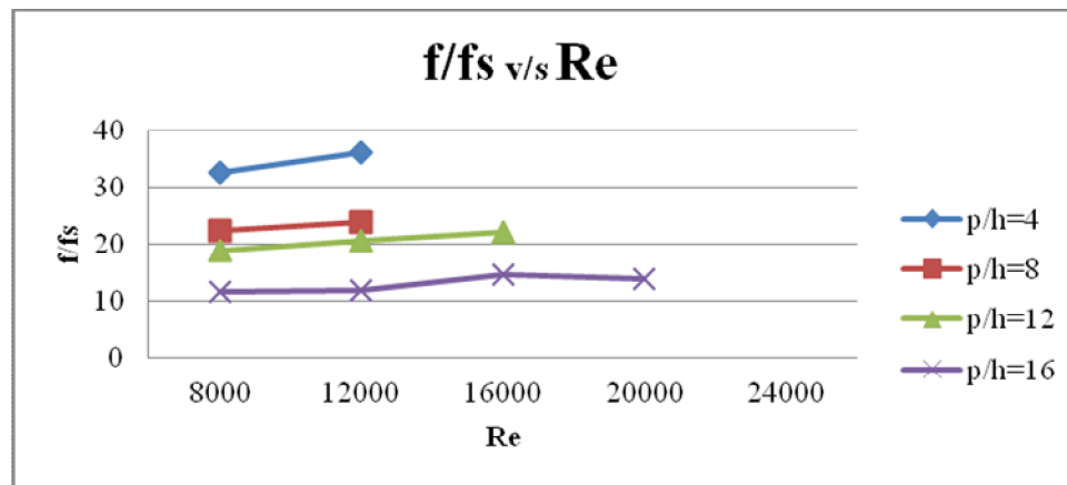
Fig 9: Variation of f/fs with Re (AR=5, h=15mm), Detachment=4mm
