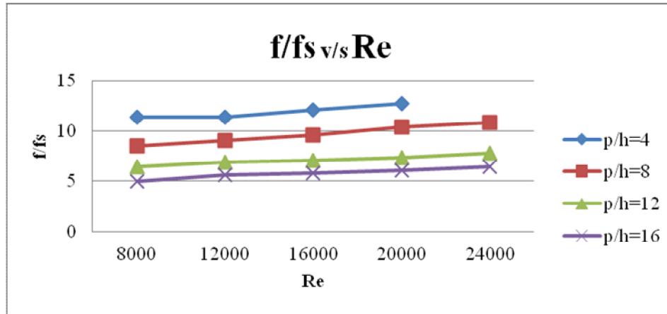
Fig 8: Variation of f/fs with Re (AR=3, h=10mm), Detachment=4mm
