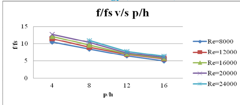
Fig. 5 : Variation of f/fs with p/h (AR=3, h=10mm), Detachment=4mm
